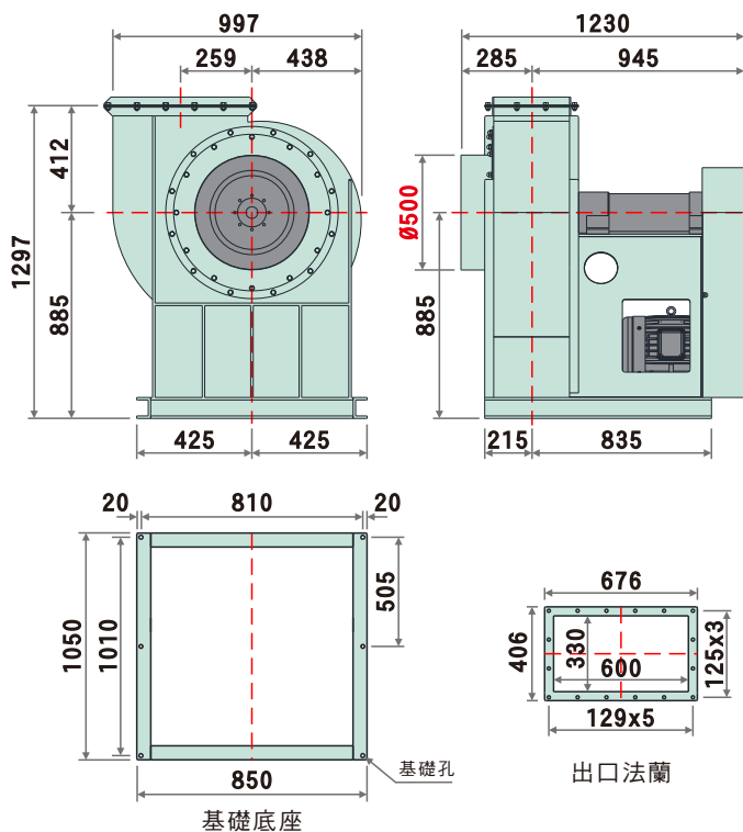
裝配方向視圖與尺寸 (DIMENSIONS)
